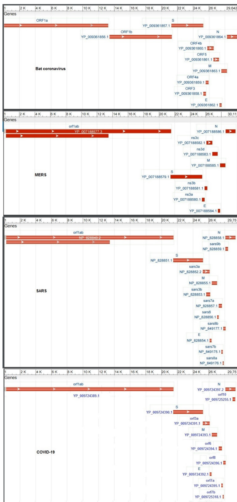
Figure 1. Protein domains of the family Coronaviridae was reconstructed for Bat Coronavirus, MERS, SARS and COVID-19 by NCBI genome viewer
