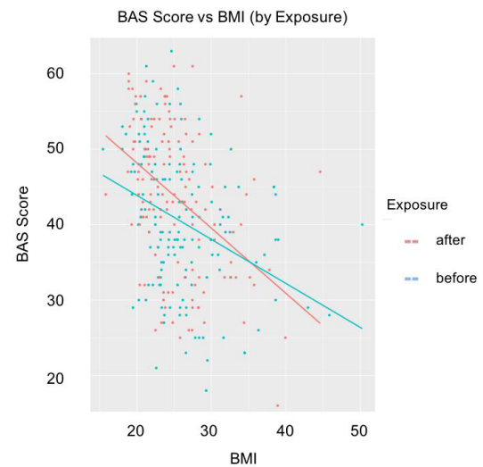
Figure 2. BAS Score vs. BMI: Both exposures resulted in a statistically significant decrease in BAS score as BMI increased ( p=8.17e-08 ); however, there is no significant difference seen between the different exposure times.
