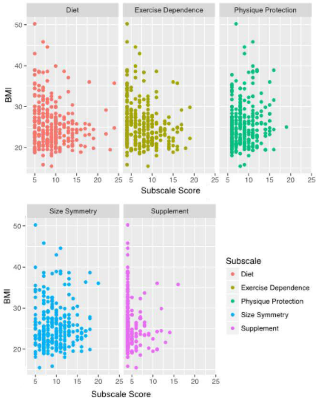
Figure 11. BMI vs. Subscales: As the BMI increased, the Diet Subscale score significantly decreased and Physique Protection Subscale scores increased. Diet ( p=0.00241 ), Physique Protection ( p=0.0374 ). Participants with higher BMIs were more likely to score a “response > 4” on the Supplement Subscale ( p=0.00927 ).
