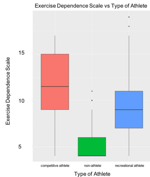
Figure 6. Exercise Dependence Subscale Score vs. Type of Athlete: Competitive athletes scored significantly higher than non-athletes on the Exercise Dependence Subscale ( p=0.0409 ).
