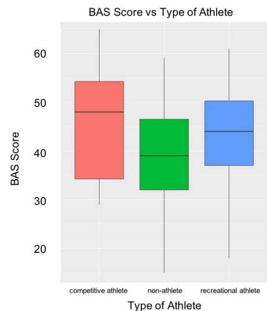
Figure 3. BAS Score vs. Type of Athlete: Non-athletes scored significantly lower on the BAS than competitive athletes ( p=0.027280 ).
