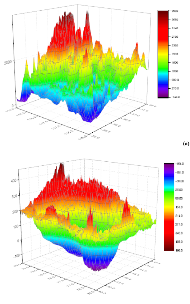
Figure 2. 3D Simulation of (a) FT-IR spectrum and (b) Raman spectrum of Cholera Toxin
