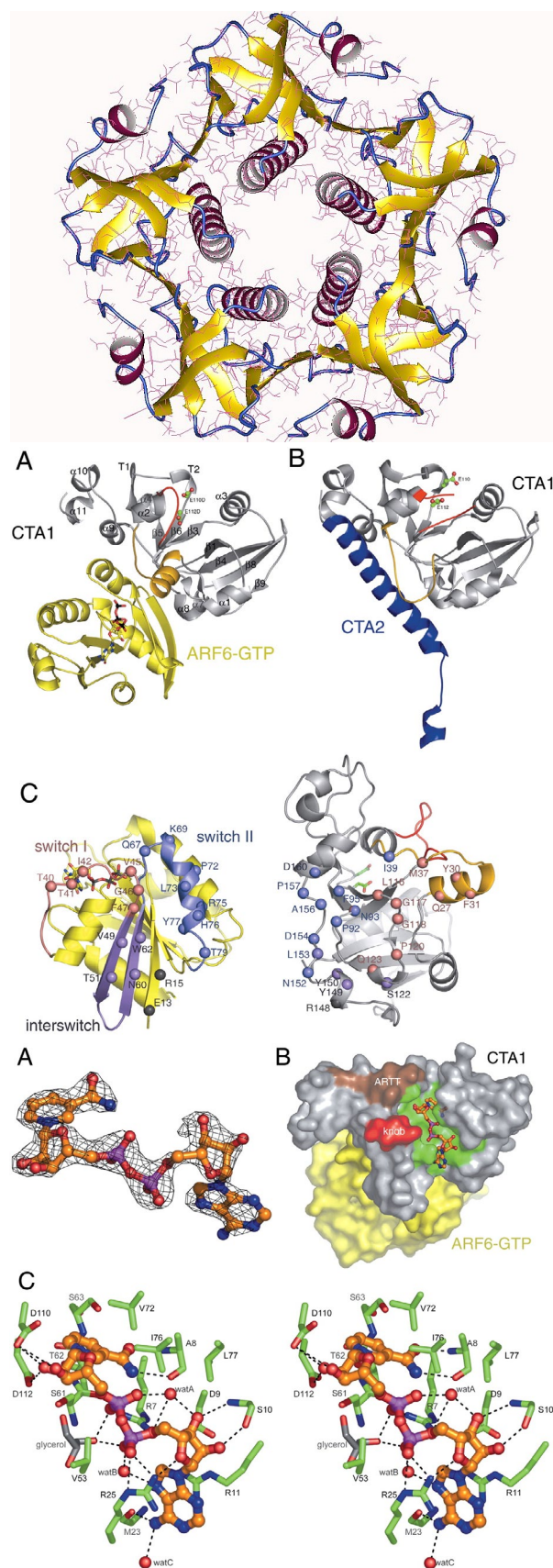
Figure 1. Different sections of the Cholera Toxin [43-93]
