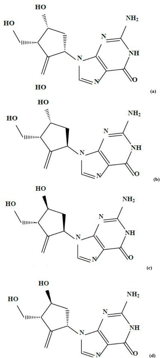
Figure 1. Molecular structure of (a) 2-Amino-9-((1S, 3R, 4R)-4-Hydroxy-3-(Hydroxymethyl)-2-Methylenecyclopentyl)-1H-Purin-6(9H)-One, (b) 2-Amino-9-((1R, 3R, 4R)-4-Hydroxy-3-(Hydroxymethyl)-2-Methylenecyclopentyl)-1H-Purin-6(9H)-One, (c) 2-Amino-9-((1R, 3R, 4S)-4-Hydroxy-3-(Hydroxymethyl)-2-Methylenecyclopentyl)-1H-Purin-6(9H)-One and (d) 2-Amino-9-((1S, 3R, 4S)-4-Hydroxy-3-(Hydroxymethyl)-2-Methylenecyclopentyl)-1H-Purin-6(9H)-One Nano molecules
