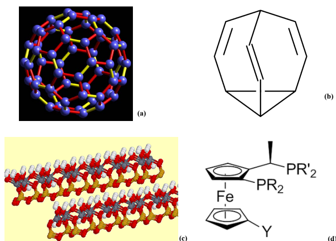
Figure 1. Molecular structure of (a) Buckminsterfullerene (Fullerene), (b) Bullvalene, (c) Dickite and (d) Josiphos Ligands Nano molecules
