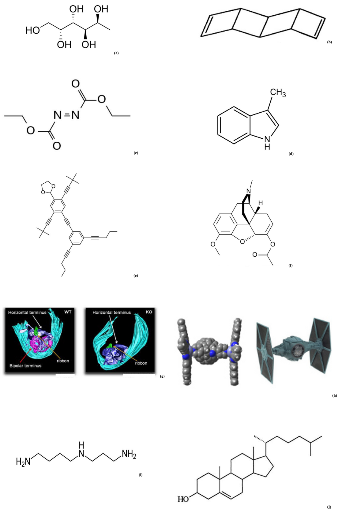
Figure 1. Molecular structure of (a) Fucitol, (b) Pterodactyladiene, (c) DEAD or DEADCAT (DiEthyl AzoDiCarboxylaTe), (d) Skatole, (e) the NanoPutians, (f) Thebacon, (g) Pikachurin, (h) Tie Fighter, (i) Spermidine and (j) Mirasorvone Nano molecules
