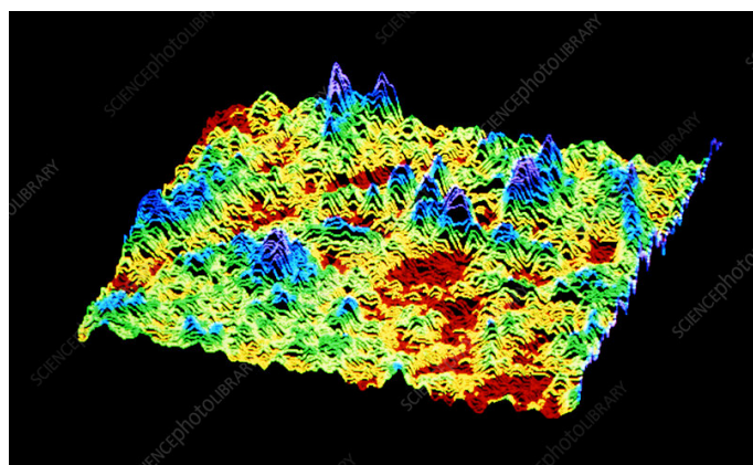
Figure 6. Extinction cross section area for Lutetium nanorods with effective radius of 45 (nm) and various dimension ratios
