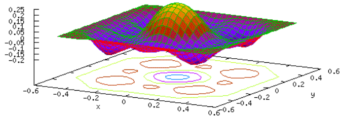
Figure 6. Extinction cross section area for Meitnerium nanorods with effective radius of 45 (nm) and various dimension ratios
