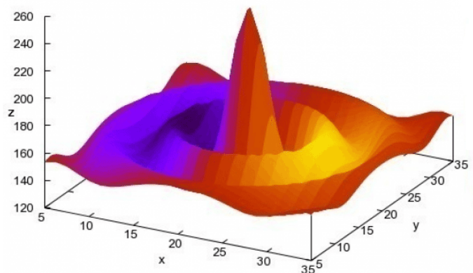
Figure 7. Maximum increase in temperature for nanorods with effective radius of 20 and 45 (nm) and various dimension ratios
