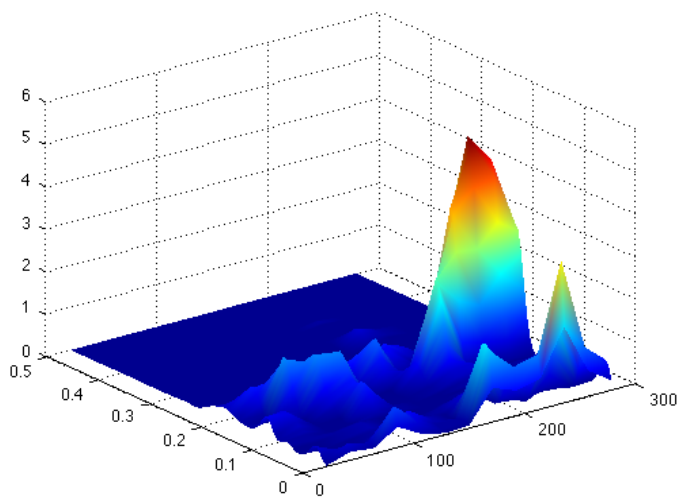
Figure 3. Maximum increase in temperature for spherical nanoparticles with radius of 45 (nm) at Plasmon wavelength of 685 (nm)
