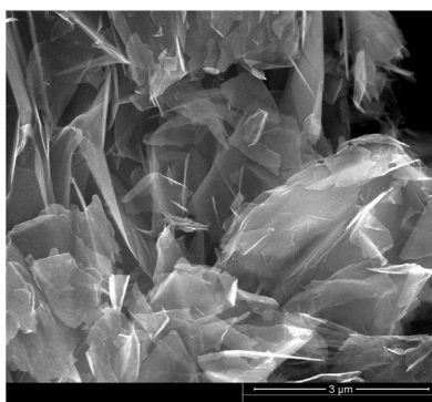
Scanning Electron Microscope (SEM) image of Lawrencium nanoparticles with 50000x zoom.
