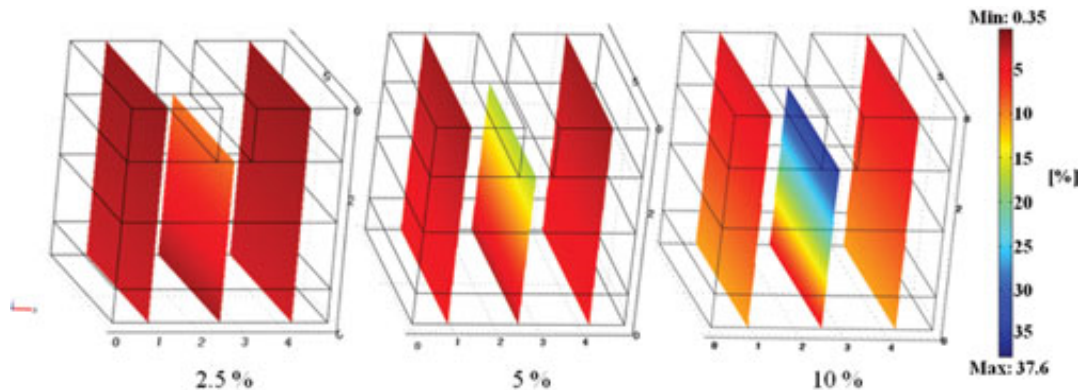
Figure 4. Maximum increase in temperature for core-shell Curium nanospheres with various thicknesses of silica shell
